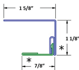
Snap J channel
