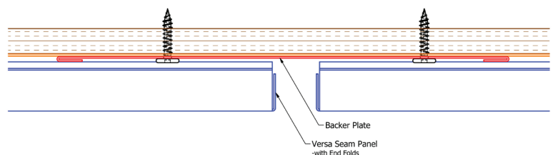
Optional end folds
